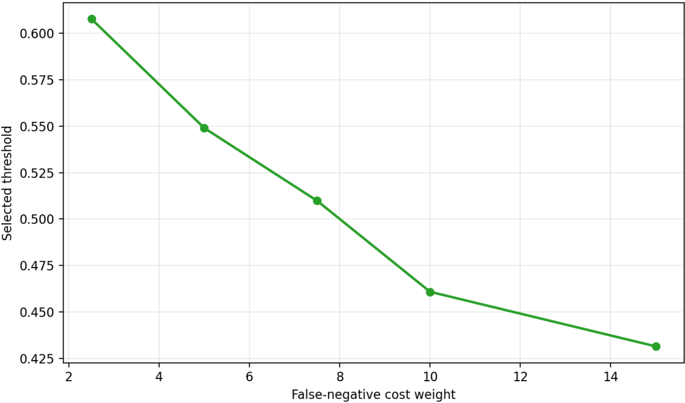
Threshold Sensitivity to Cost Weights
