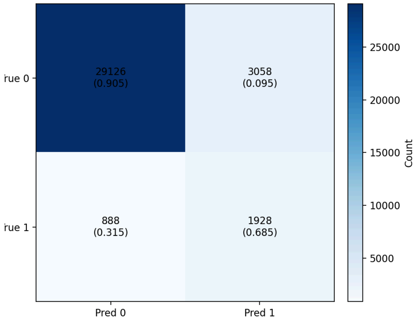
Train Confusion Matrix (threshold=0.549)
