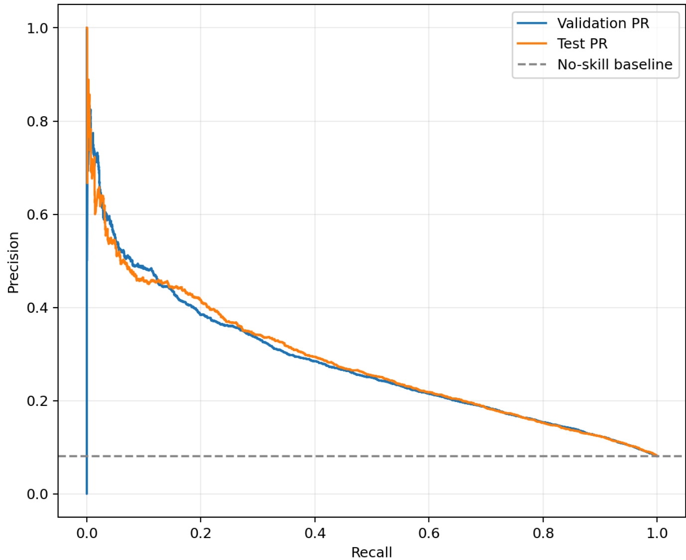
Precision-Recall Curves (Validation and Test)
