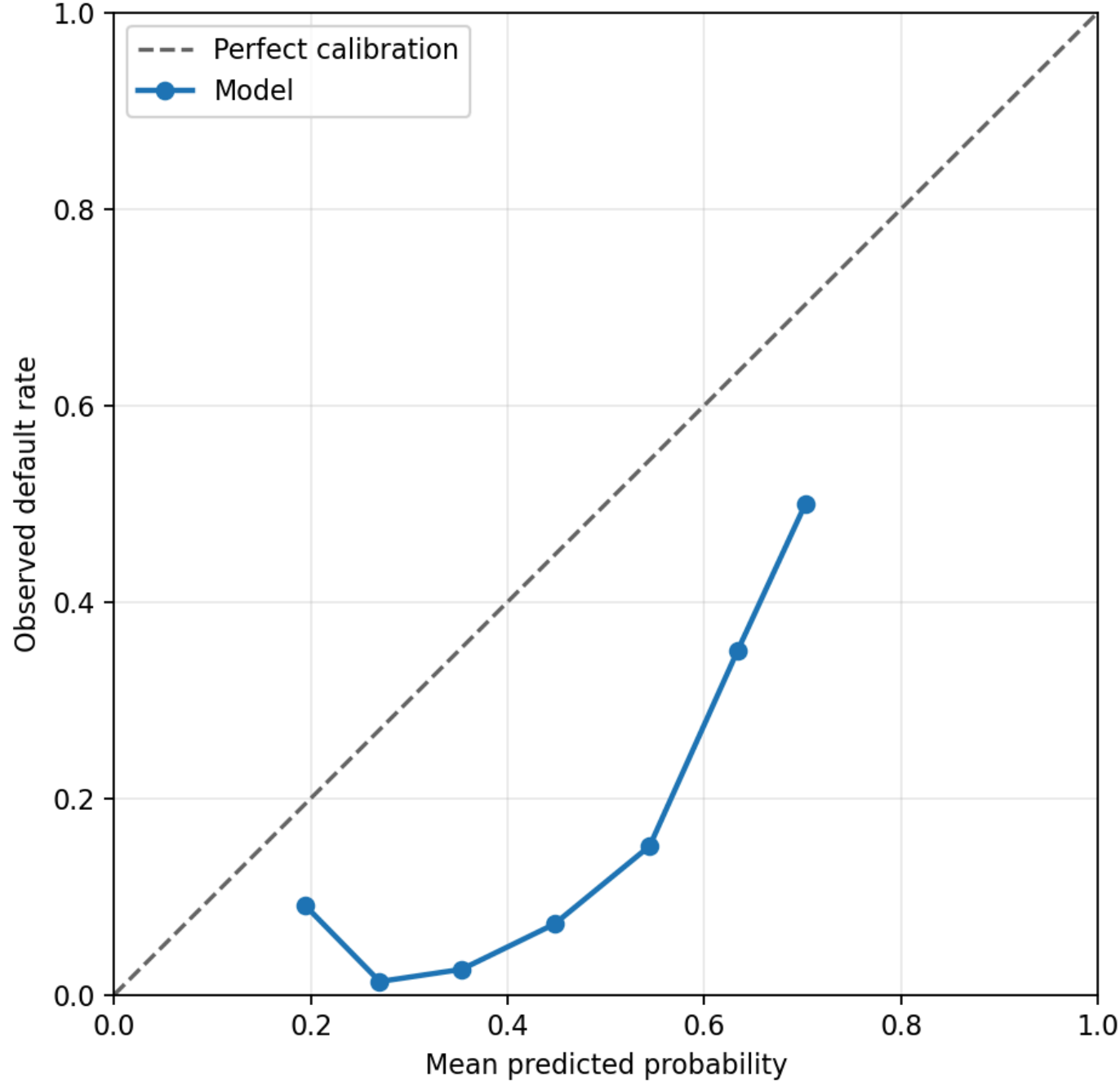
Validation Calibration Curve
