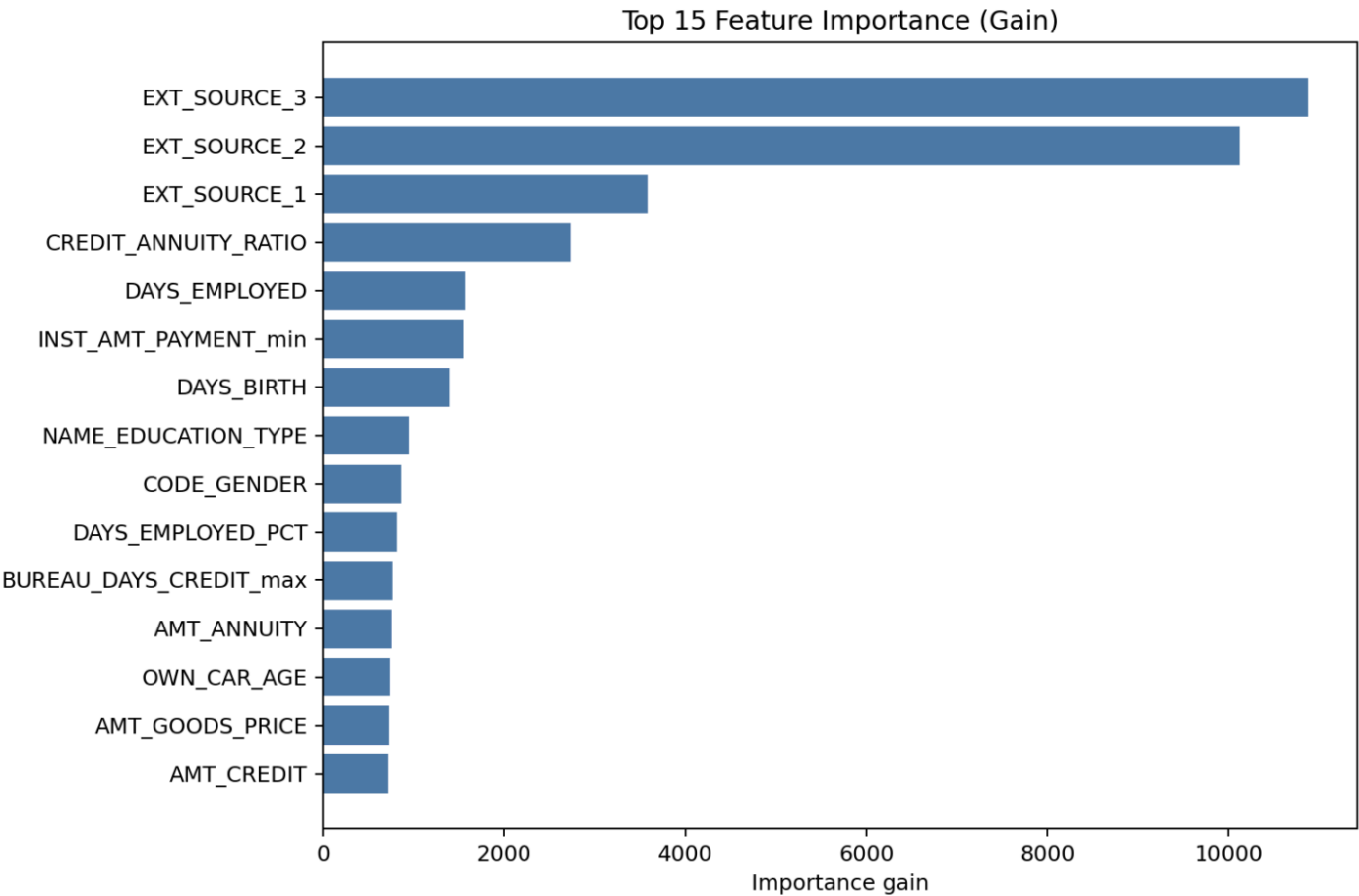
figure7_top15_feature_importance.png
