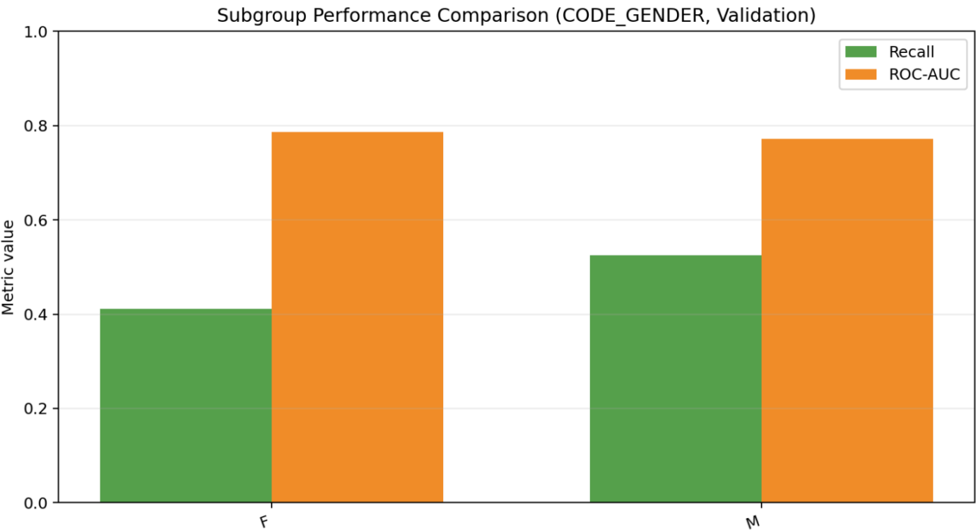
figure6_subgroup_performance_comparison_validation.png
